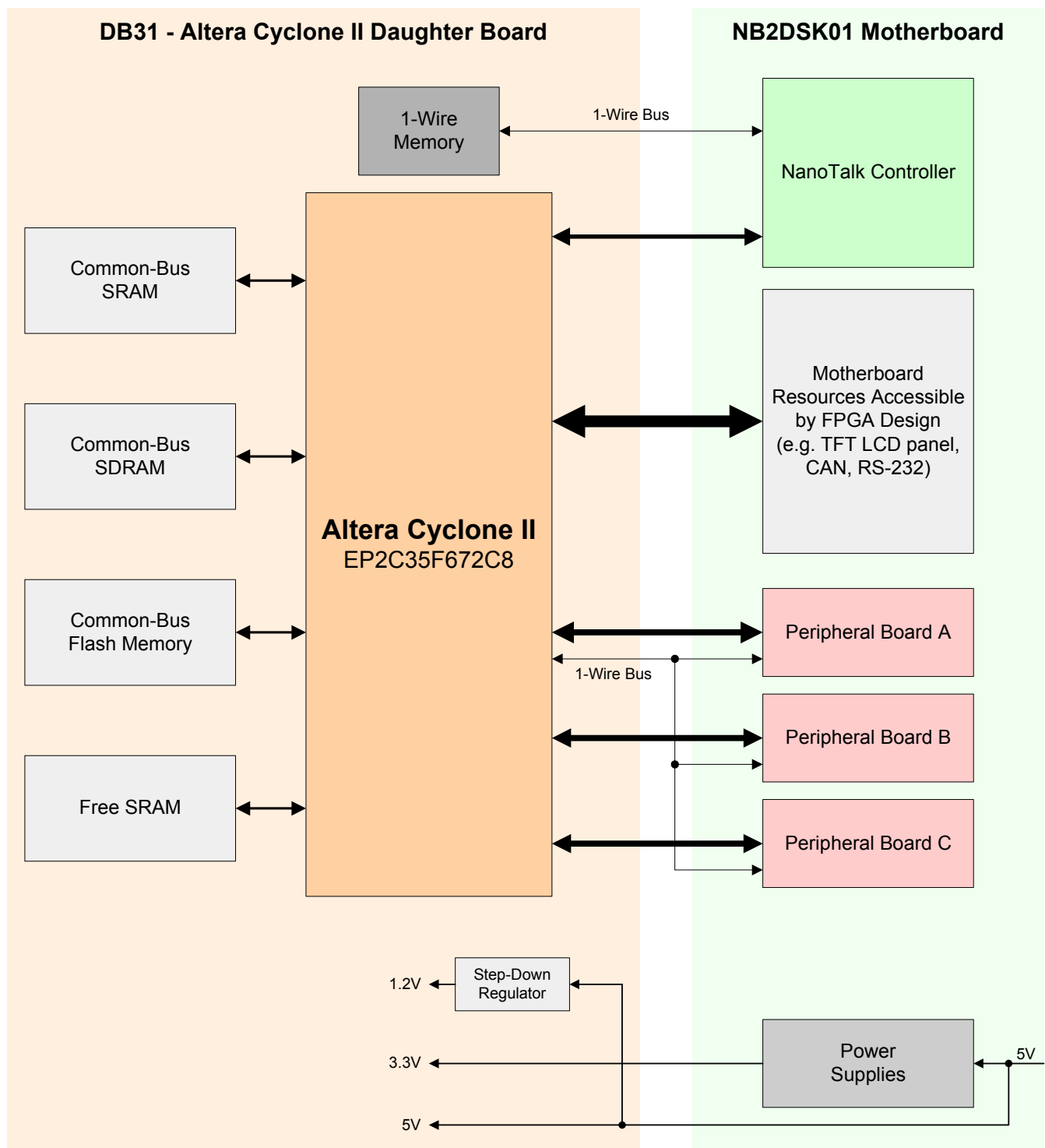
Figure 2. Altera Cyclone II daughter board (DB31) block diagram.
